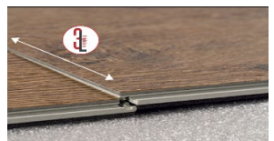
Figure 5: Slide plank 3 to your left until the short side is in contact with the short side of plank 1. Drop the short side of plank 3 onto the short side of plank 1 making sure that there is no gap between the short side of plank 1 and plank 3.
